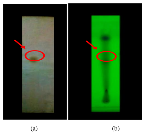
Figure 1. TLC chromatogram in (a) visible light, (b) UV (366 nm) for the samples of EAT, arrows indicate flavanoids component.
